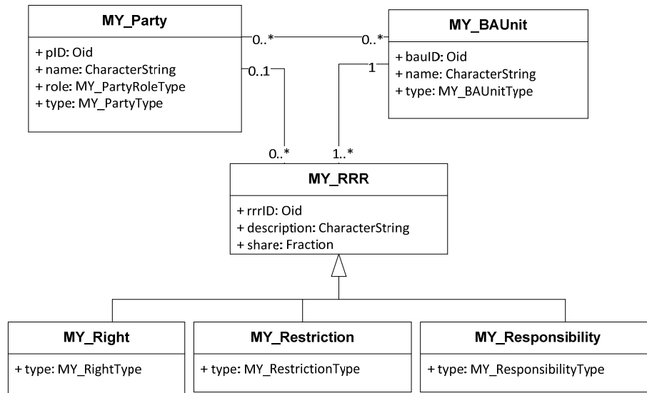
Figure 2: Non-spatial data modelling based on LADM.
