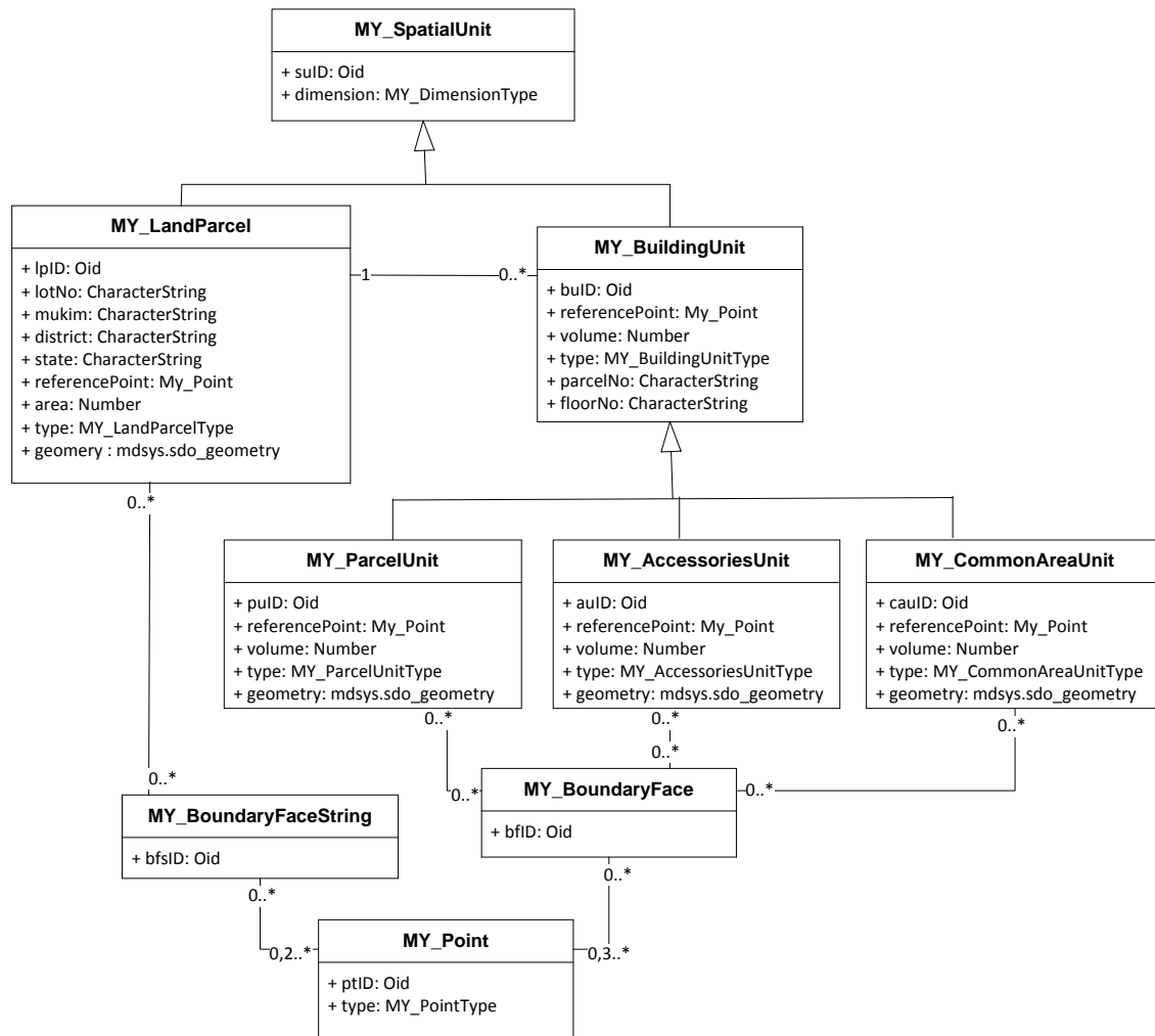
Figure 1: Spatial data modelling based on LADM
