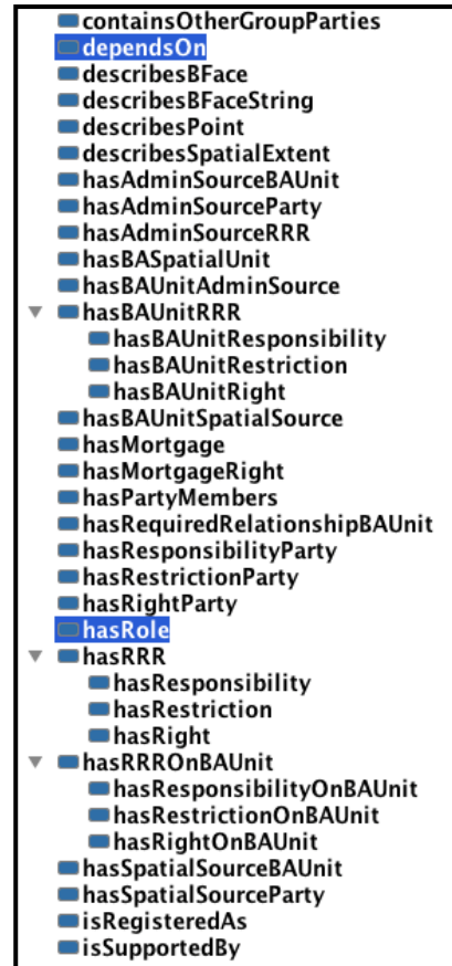
(c) Object Properties
